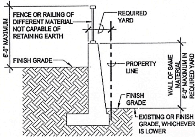
RETAINING WALLS WITH SAFETY RAILINGS
