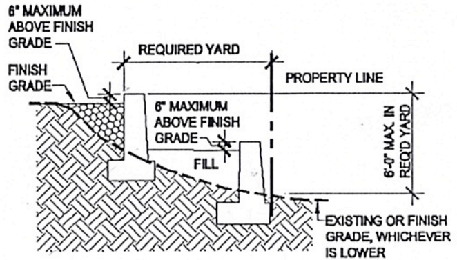
TERRACED RETAINING WALLS
