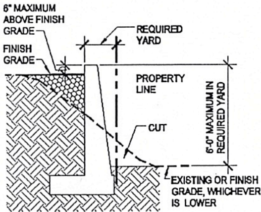
CUT and FILL RETAINING WALL
