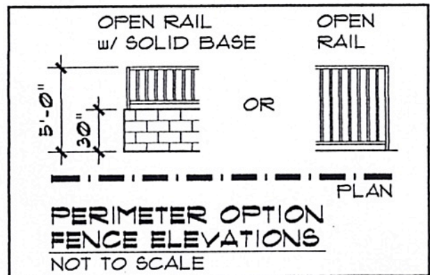
SKETCH "F"
