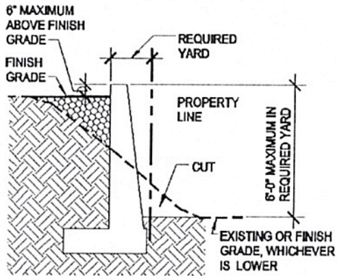
CUT and FILL RETAINING WALL
