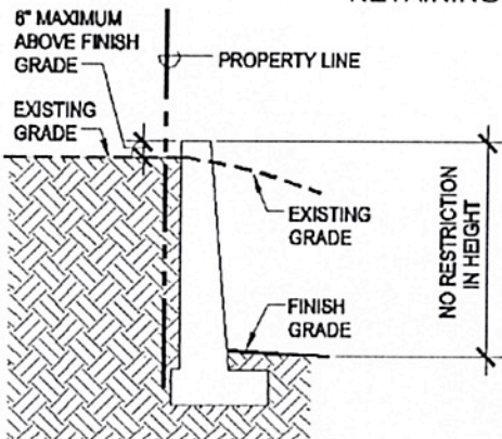
RETAINING WALL PROTECTING A CUT
