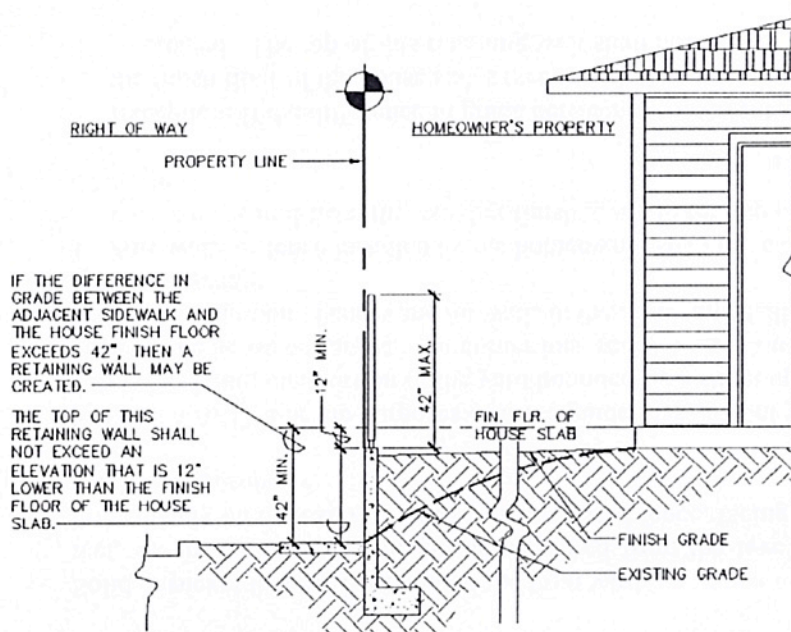
Sketch "C"
