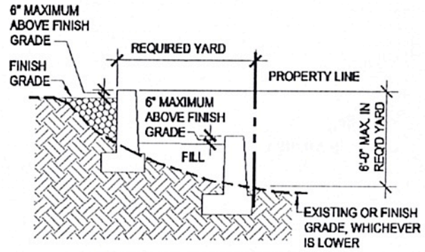
TERRACED RETAINING WALLS
