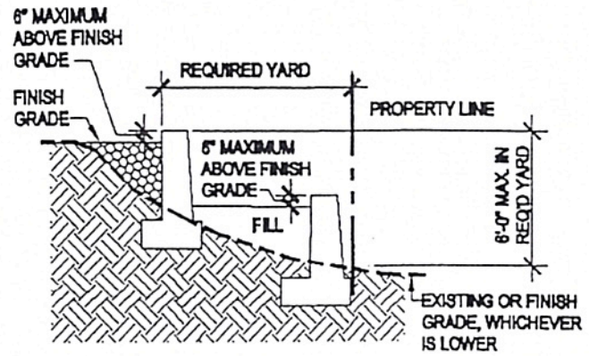
TERRACED RETAINING WALLS
