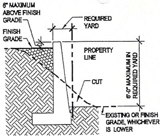
CUT and FILL RETAINING WALL
