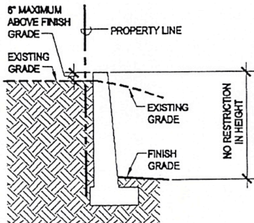
RETAINING WALL PROTECTING A CUT
