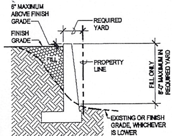
RETAINING WALL CONTAINING FILL
